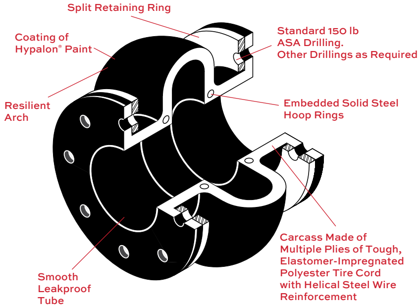
1 ARCH Style 1001 High Movement Expansion Joint
