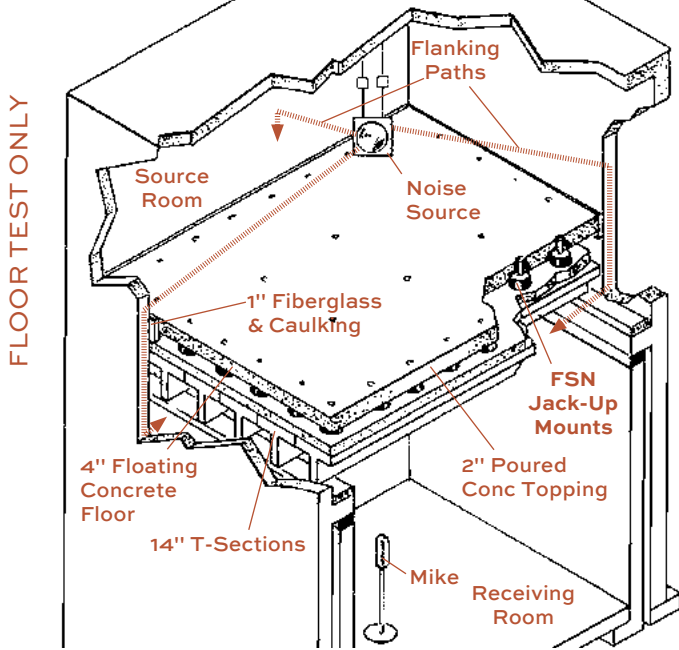
FIRST TEST in March 1971 of a floating floor only. Disappointing results because of flanking problems down the walls.
