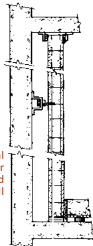
Structural Floor Supported Wall
