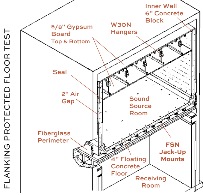
SECOND TEST in June 1971 of same floating floor with isolated walls and ceiling to prevent flanking. Basically room within a room construction.
