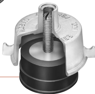
M. Type FSN LDS Jack-Up Mount
