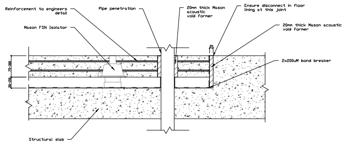
FSN 04 TYPICAL DETAIL - FSN RUBBER JACK UP FLOOR NTS - With Pipe Penetration
