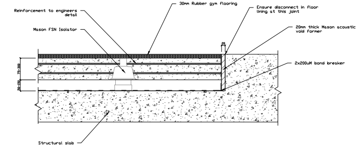
FSN 06 TYPICAL DETAIL - FSN RUBBER JACK UP FLOOR NTS - With Gym Flooring
