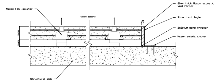
FSN 02 TYPICAL DETAIL - FSN RUBBER JACK UP FLOOR ALT HOB NTS
