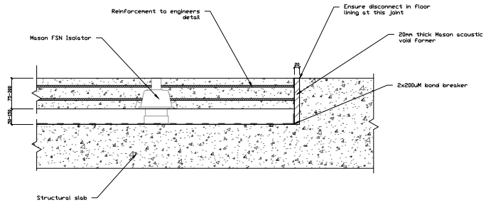
FSN 01 TYPICAL DETAIL - FSN RUBBER JACK UP FLOOR NTS
