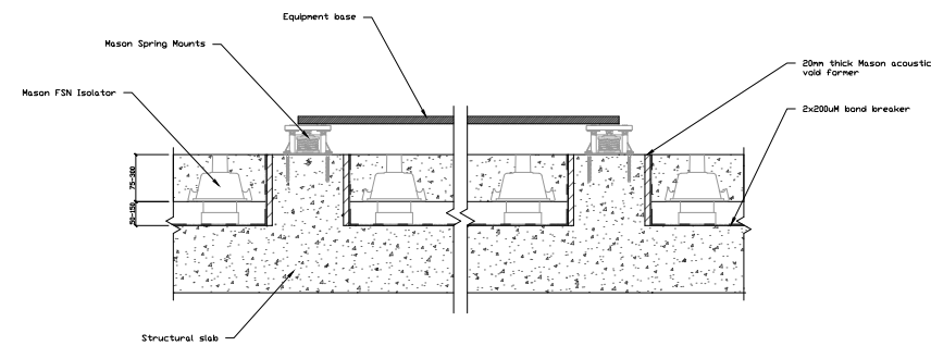
FSN 05 TYPICAL DETAIL - FSN RUBBER JACK UP FLOOR ALT HOB NTS - With Equipment Plinths
