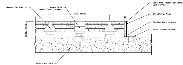
FSN 03 TYPICAL DETAIL - FSN RUBBER JACK UP FLOOR ALT HOB NTS - With Seismic Restraint
