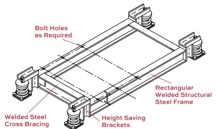
WF STEEL BEAM BASE
