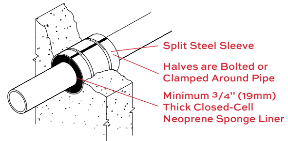
SWS WALL SEAL
