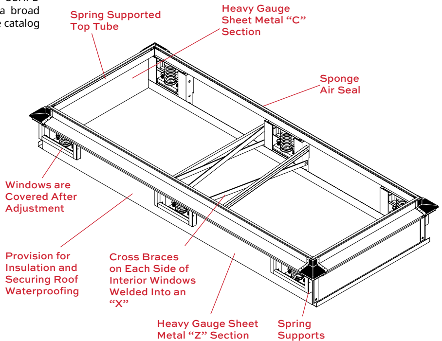
RSC COMPLETE ROOFTOP SPRING CURB
