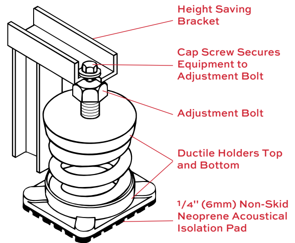
SLF SPRING MOUNT
