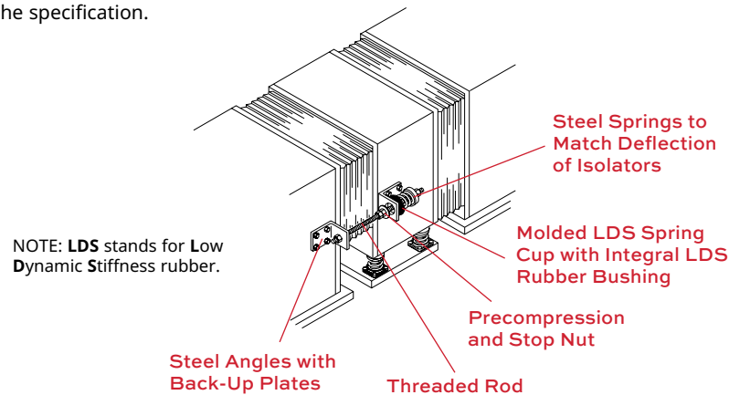
WB HORIZONTAL THRUST RESTRAINTS
